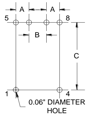
Board Layout
