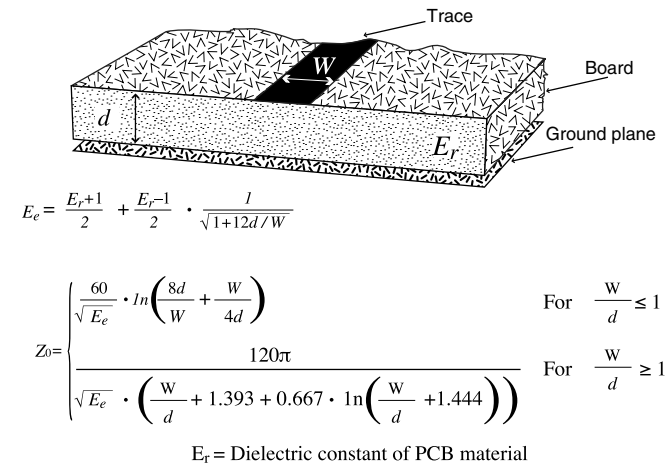
Figure 52: Microstrip Formulas
